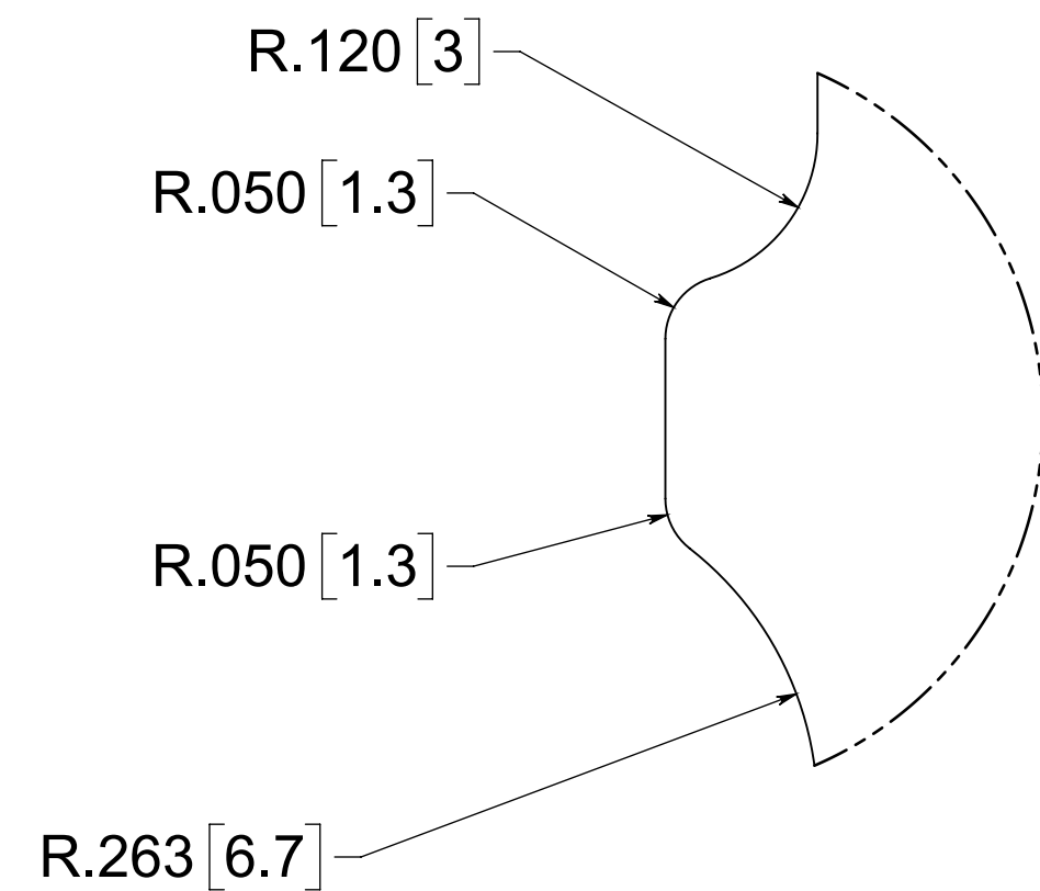
DETAIL C SCALE 6 : 1
