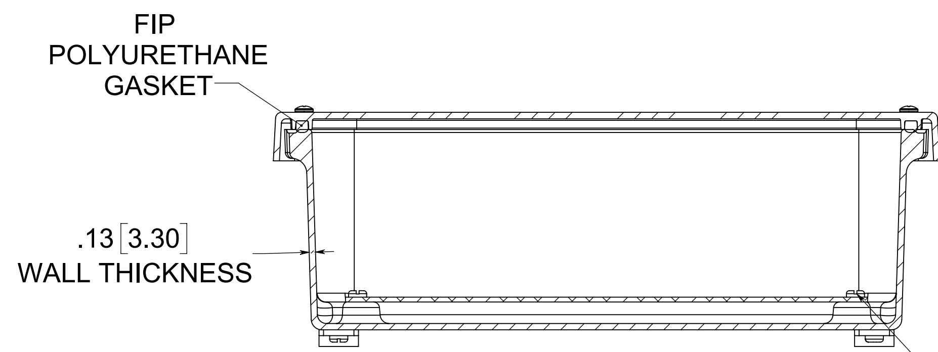
SECTION B-B
