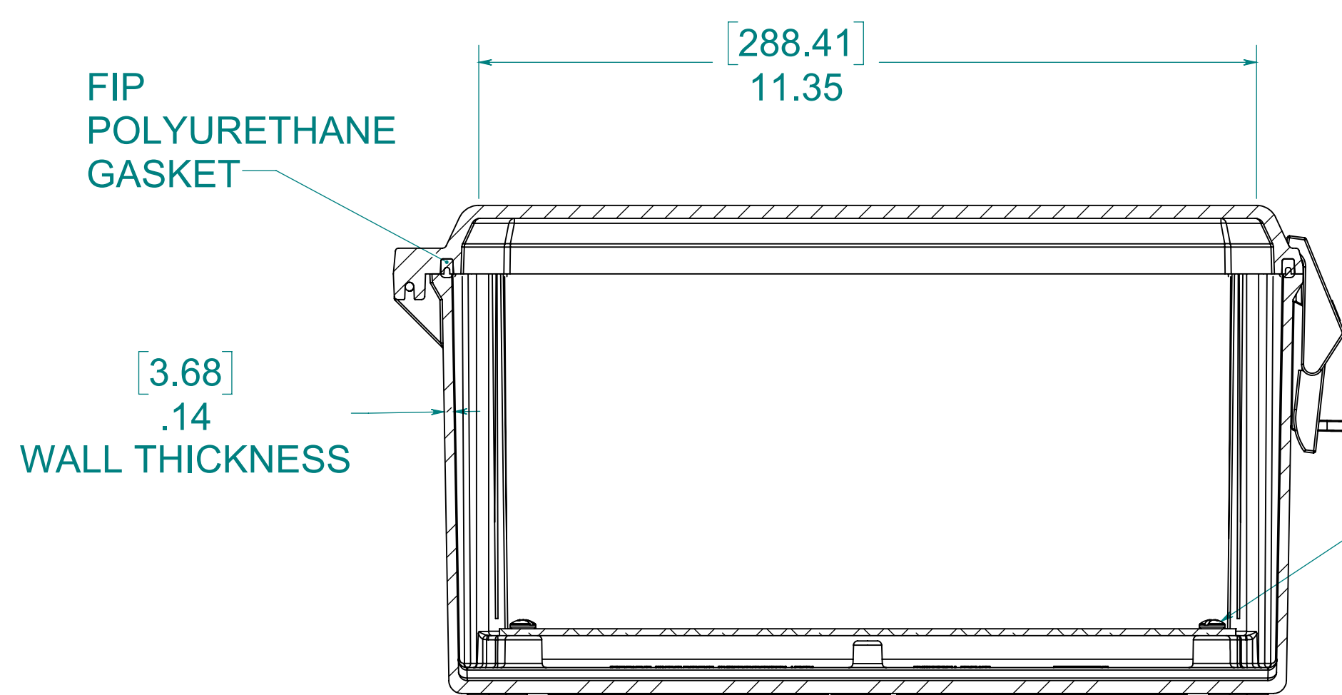
SECTION B-B
