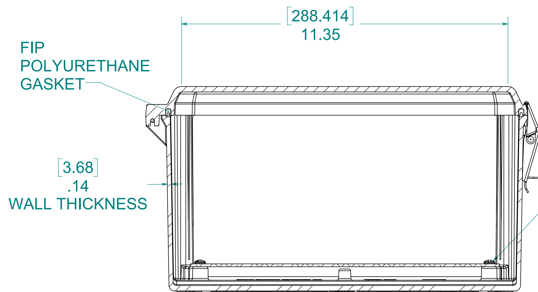
SECTION B-B
