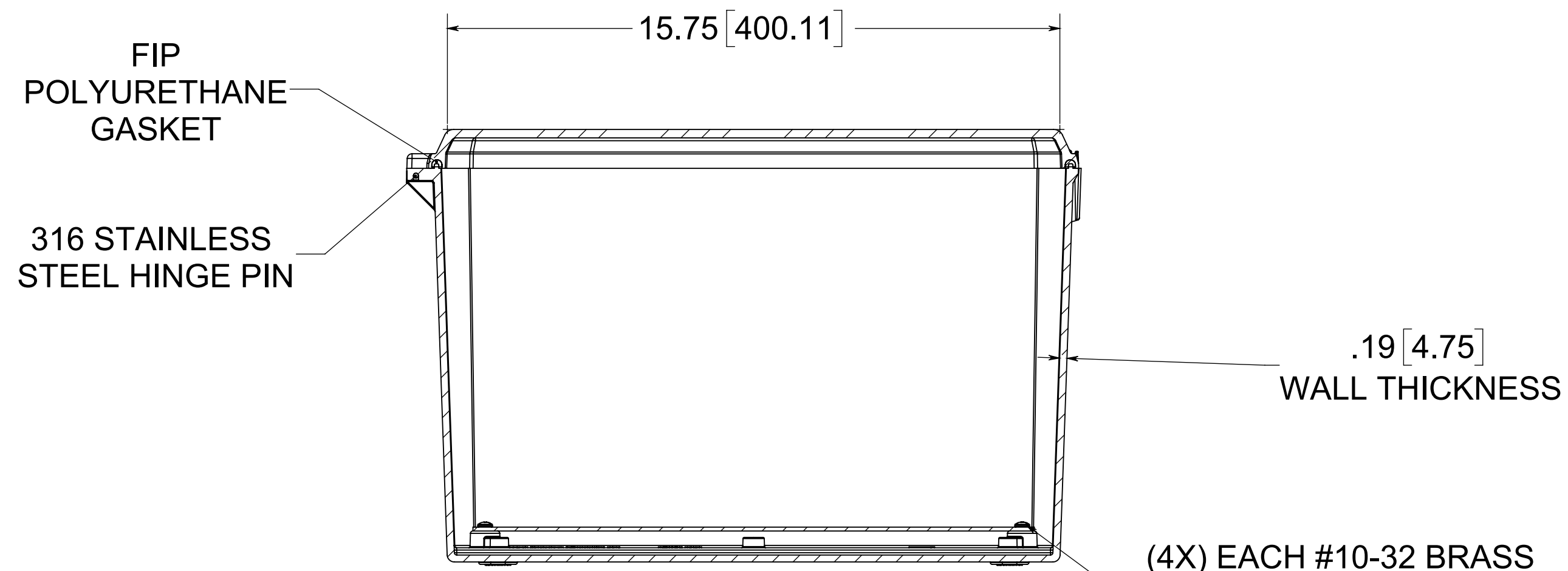
SECTION C-C
