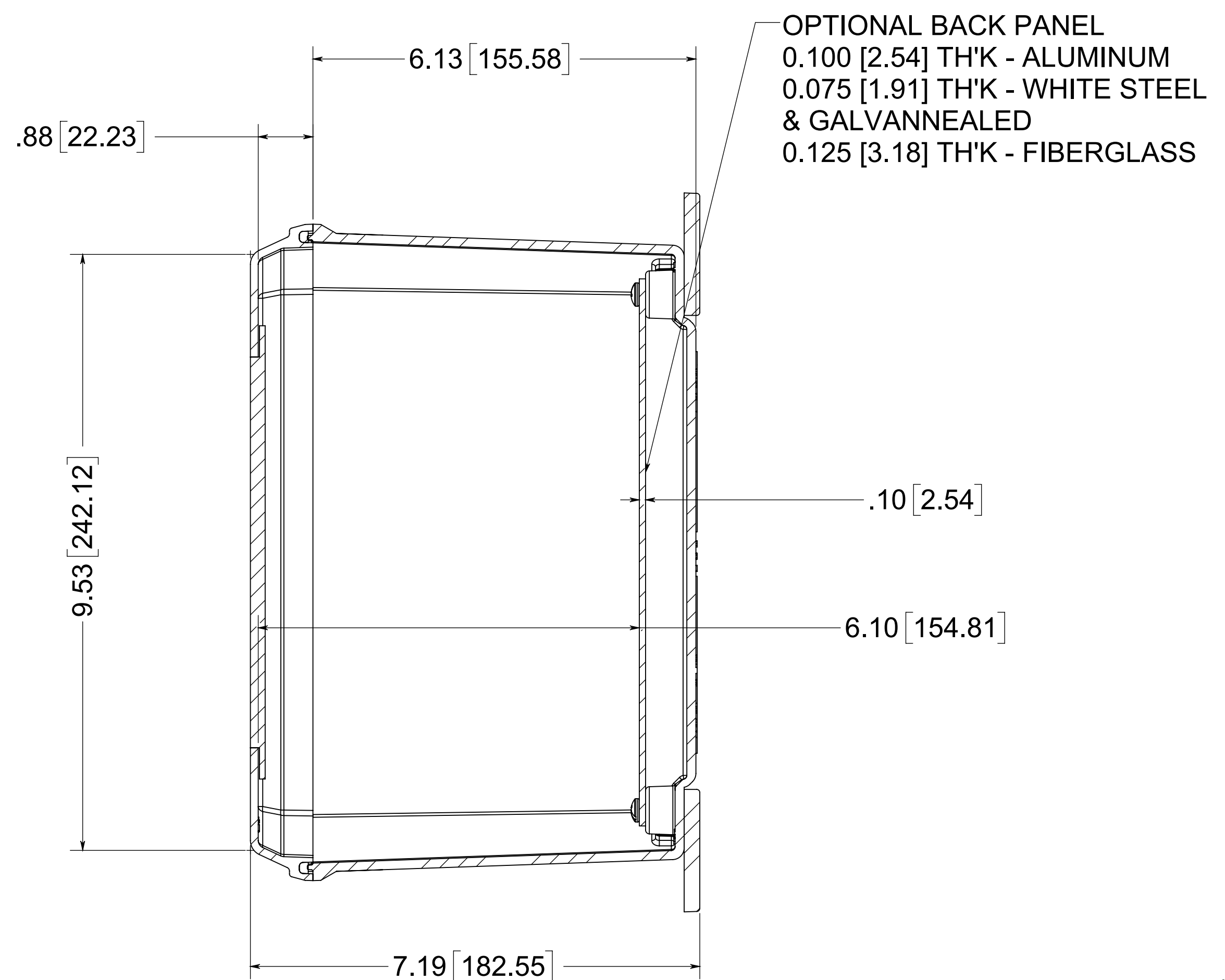
SECTION B-B
