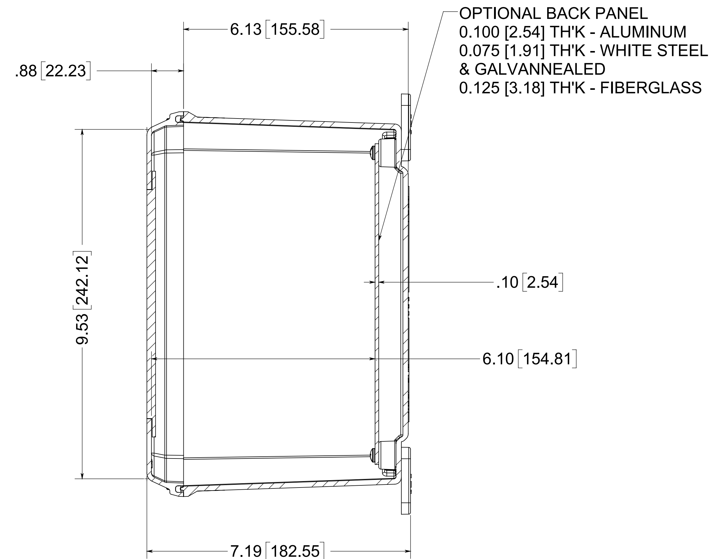
SECTION B-B
